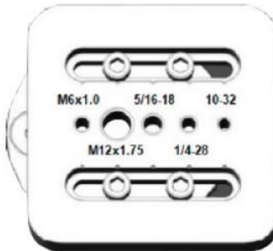
Multi-Thread Plate SPK-TCM-005
